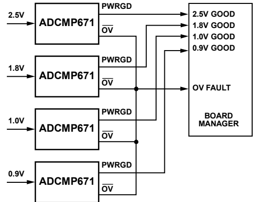
Figure 35. N Rails Monitoring with N + 1 Processor I/O
