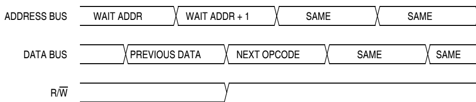
Figure 13-14. Wait Mode Entry Timing
