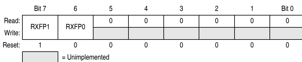
Figure 14-7. SLIC Prescale Register (SLCP)
