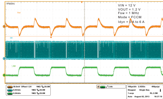
Figure 20. FCM Mode Load Transient
