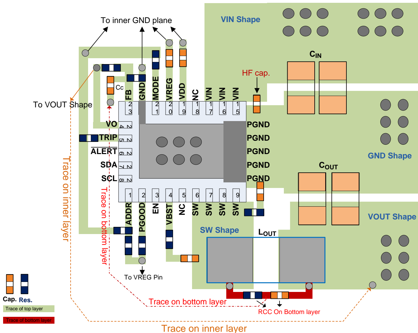
Figure 65. Layout Recommendation
