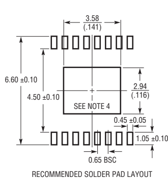
RECOMMENDED SOLDER PAD LAYOUT
