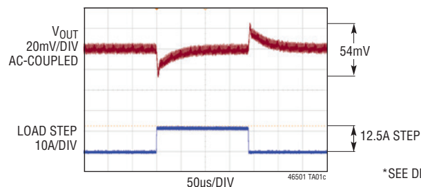
25% Load Step Transient Response, \pm 3\% Output Regulation Window. 12V IN , 1.0V OUT , 50A with 6x 220µF Ceramic Cap
