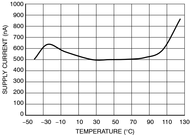
Figure 12. Power-Down Supply Current vs. Temperature
