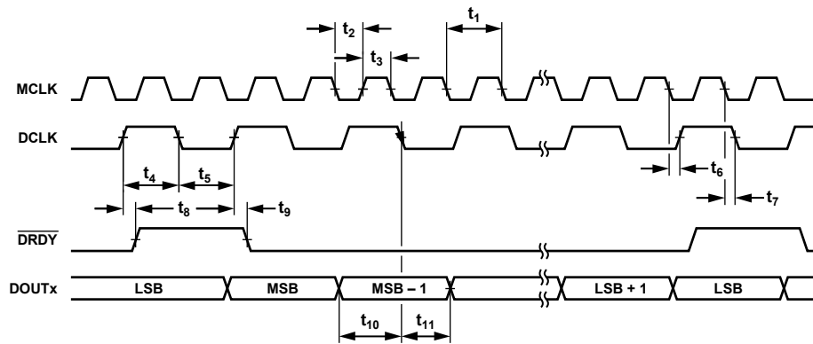
Figure 2. Data Interface Timing Diagram
