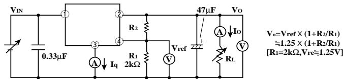
Fig.2 Test circuit for Ripple Rejection
