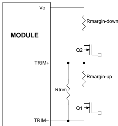
Figure 26. Circuit Configuration for margining Output voltage.
