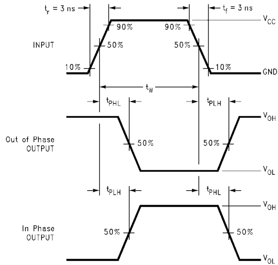
Figure 7. AC Waveforms
