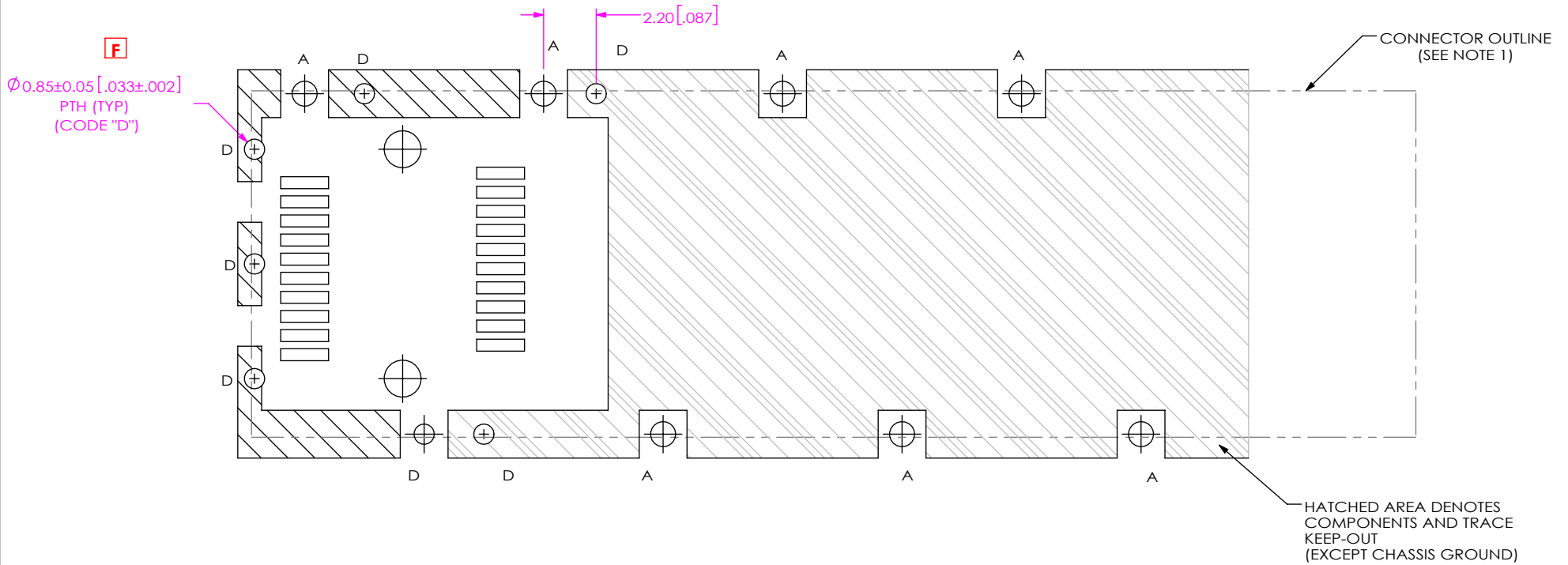
FIG 2 F SFPC-PC SHOWN (DIFFERENT AS SHOWN, OTHERWISE SAME AS FIG 1)
