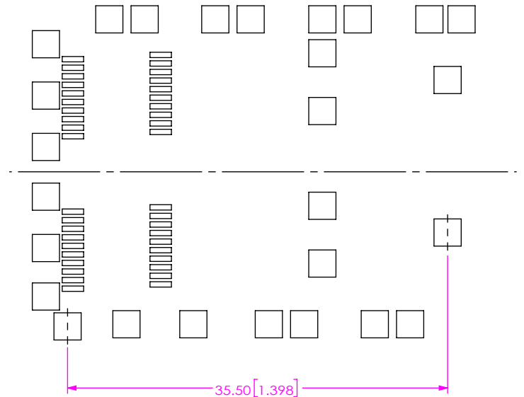
FIG 10 SFPC-2PX-XX-X SHOWN (FOR PF & PC TAILS ONLY) (DIFFERENT AS SHOWN, OTHERWISE SAME AS FIG 9)
