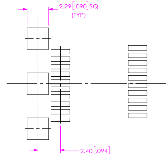
FIG 7 F SFPC-PC SHOWN (DIFFERENT AS SHOWN, OTHERWISE SAME AS FIG 6)
