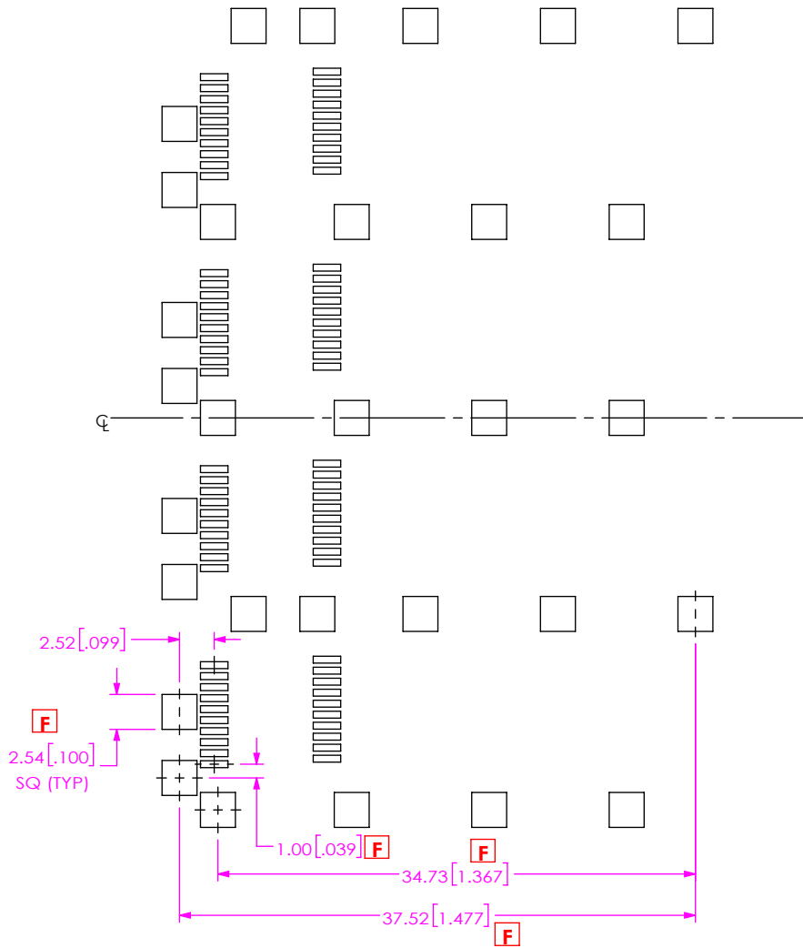
FIG 11 F SFPC-4SL-XX-X SHOWN (DIFFERENT AS SHOWN, OTHERWISE SAME AS FIG 5 & 6)
