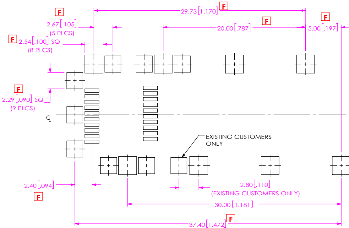
FIG 8 F SFPC-SL SHOWN (DIFFERENT AS SHOWN, OTHERWISE SAME AS FIG 3 & 6) F:\dwg\misc\mktg\footprnt\SFPC-FOOTPRINT.SLDDRW
