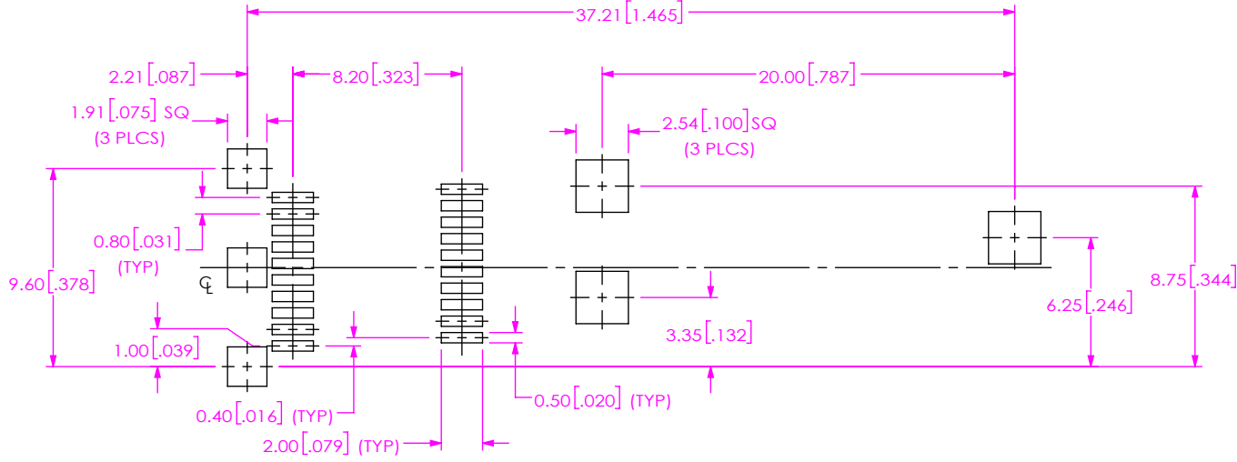
FIG 6 F SFPC-PF SHOWN (DIFFERENT AS SHOWN, OTHERWISE SAME AS FIG 1)
