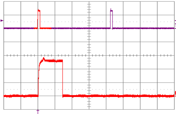
Figure 15: Load current (top trace, 20\text{ A}/\text{div.} , 50\text{ mS}/\text{div.} ) into a 10\text{ m}\Omega short circuit during restart, at V_{in} = 48\text{ V} . Bottom trace ( 10\text{ A}/\text{div.} , 5\text{ mS}/\text{div.} ) is an expansion of the on-time portion of the top trace.
