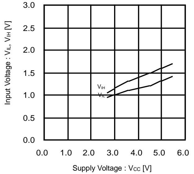
Figure 14. Input Voltage vs Supply Voltage
