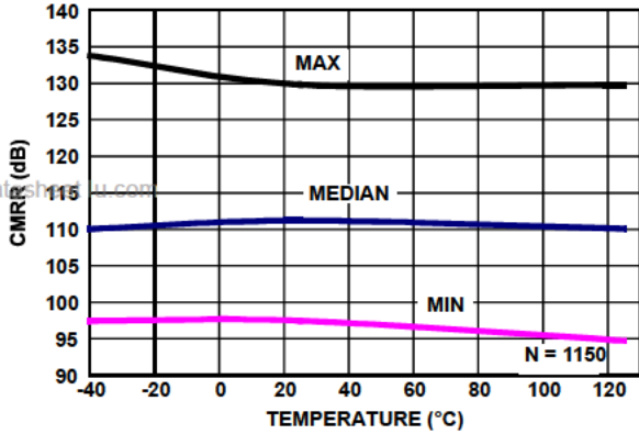
FIGURE 30. CMRR vs TEMPERATURE V_{CM} = \bar{+}2.5V \text{ TO } -2.5V, V_+, V_- = \pm 2.5V
