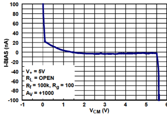
FIGURE 19. INPUT OFFSET CURRENT vs COMMON-MODE INPUT VOLTAGE
