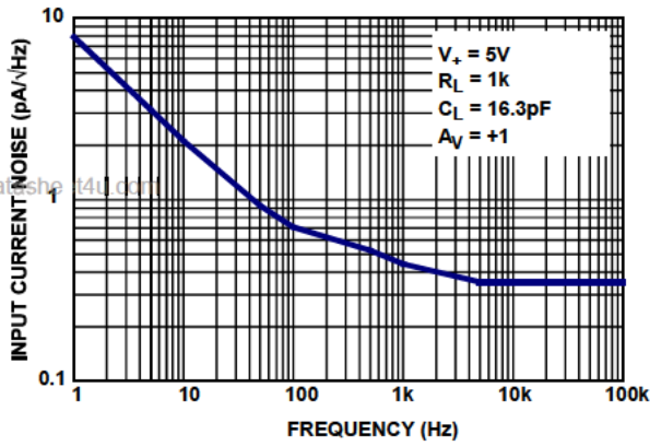
FIGURE 13. INPUT CURRENT NOISE DENSITY vs FREQUENCY
