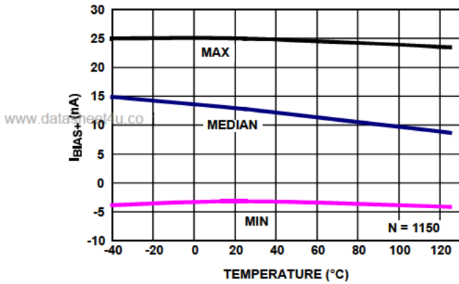
FIGURE 24. I_{BIAS+} vs TEMPERATURE, V_+, V_- = \pm 2.5V
