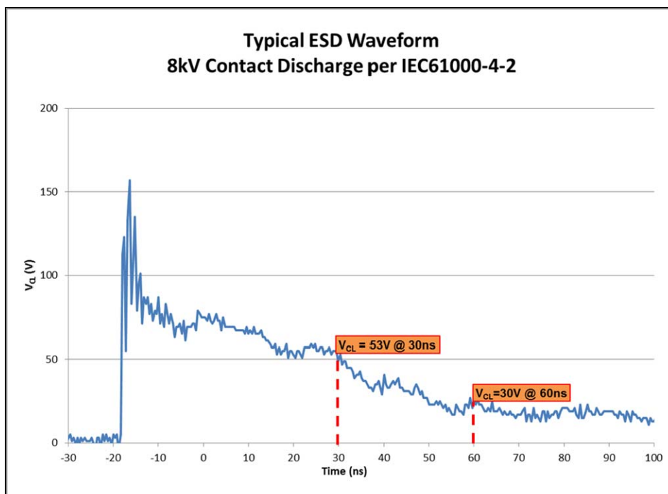
FIGURE 3. ESD WITHSTAND
