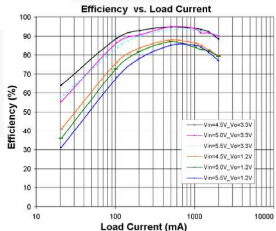
Figure 9. Power Efficiency
